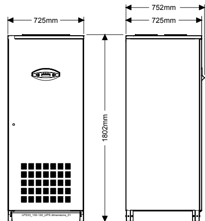
LP 33 Series / 100 & 120 kVA
