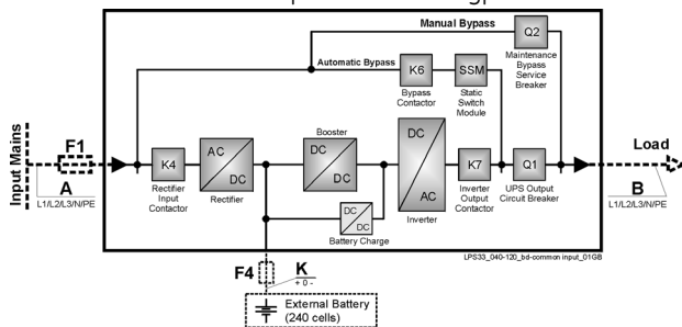
Common input Rectifier & Bypass
