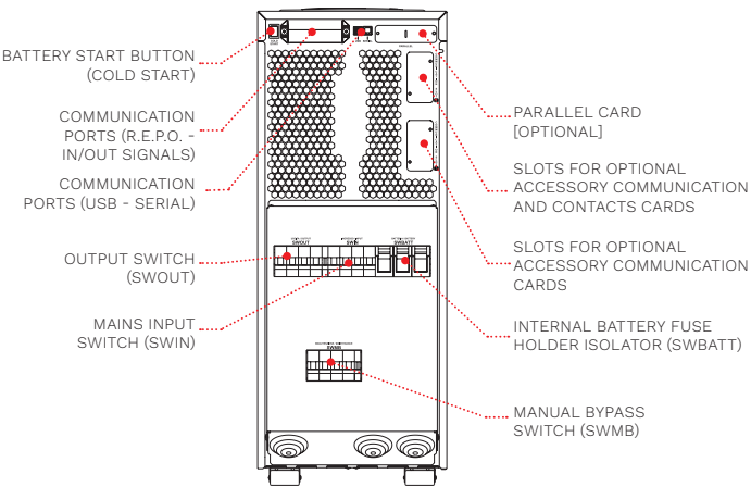
COMPACT (rear)
