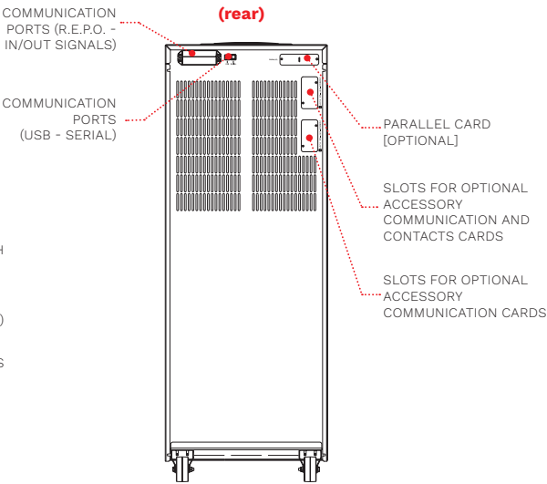
ACTIVE (rear)
