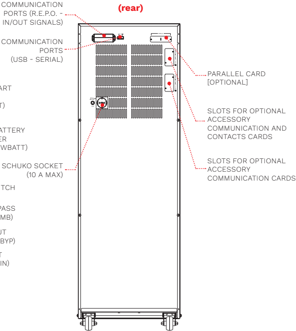
XTEND (rear)
