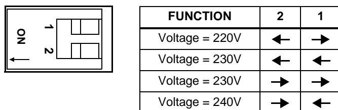
Figure 14 DIP switch settings for 230V system
